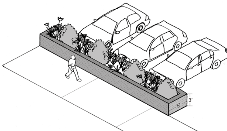
Figure 1-66. Elevated parking lot planting buffer.
