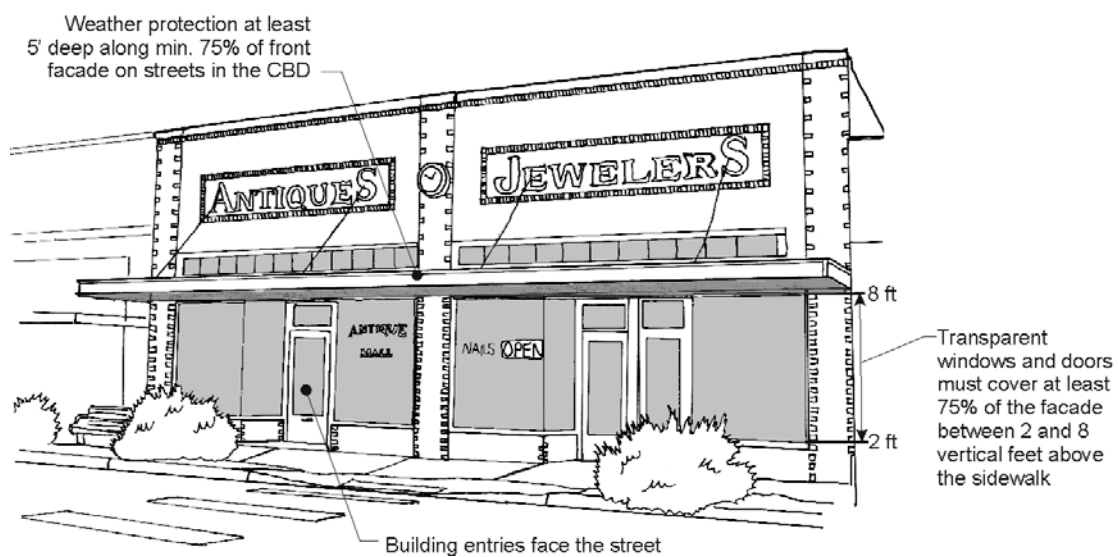
Figure 1-1. Standards for pedestrian-oriented facades.
