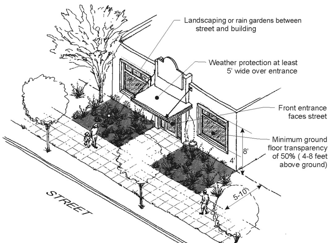
Figure 1-3. Example of landscaping in front of a building permitted for CBD properties south of Maple Street.
