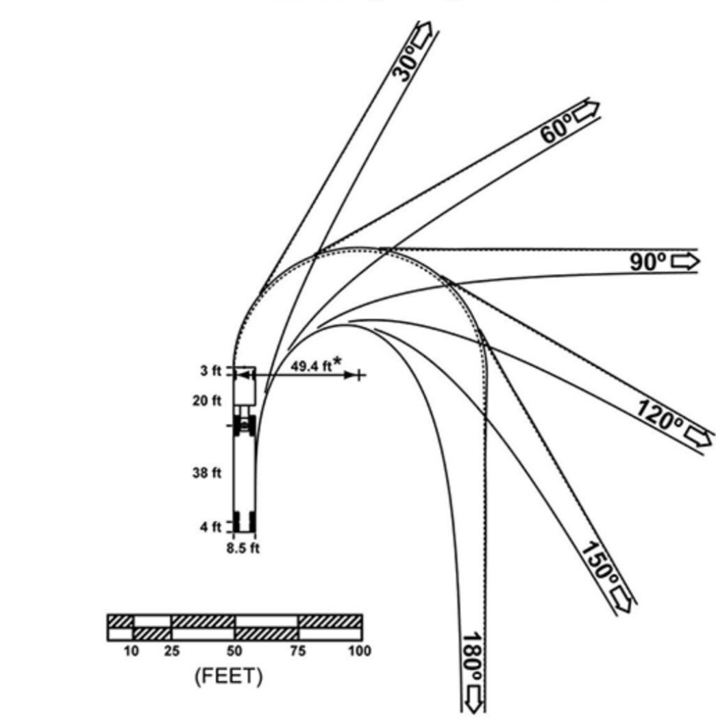
Figure 404.5C California Legal Design Vehicle 50-Foot Radius
