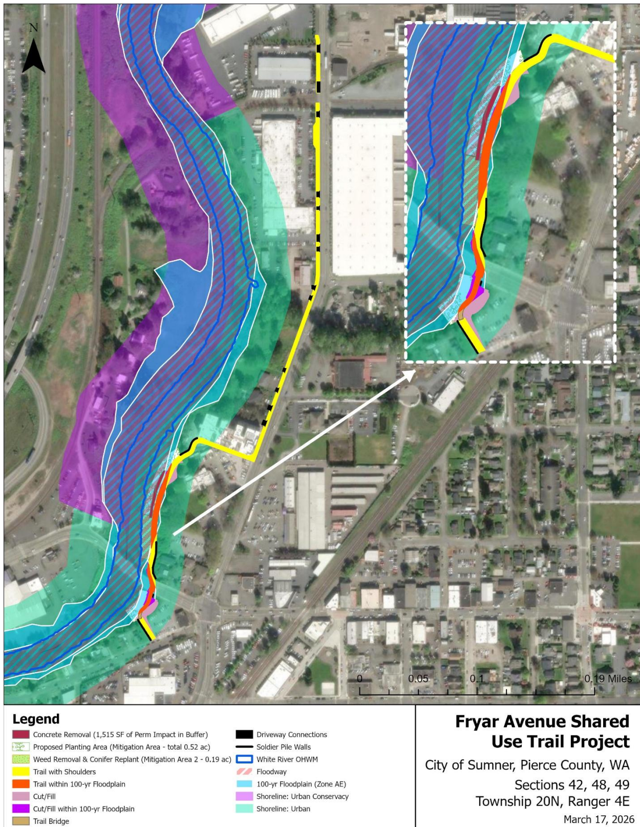
Figure 2. Shoreline Elements
